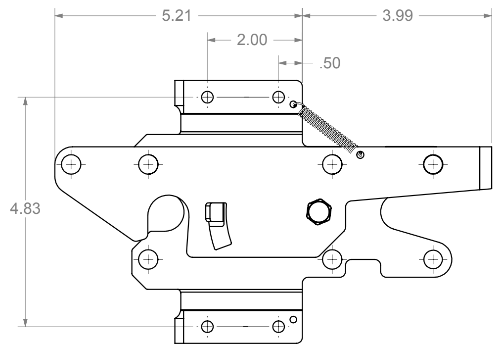
LATCH ASSEMBLY
