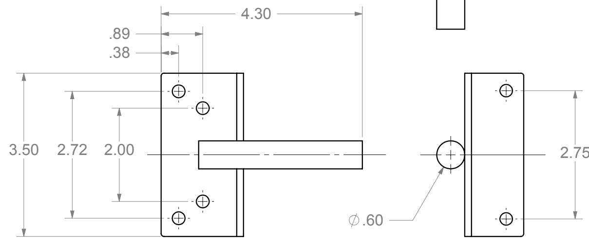
STRIKE BAR
